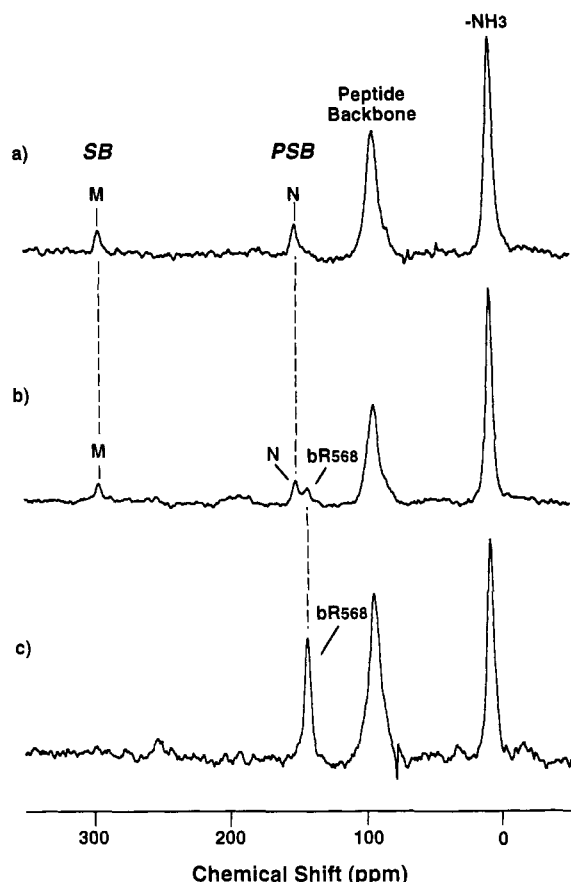
FIGURE 1: 15 N CPMAS spectra of [ε- 15 N]lysine bR, with spinning side bands suppressed by variation of the spinning speed. (a) The M and N states. (b) Products of partial thermal decay obtained when the sample containing the M and N intermediates is warmed up to -30 °C. (c) Product of further thermal decay obtained when the sample containing the M and N intermediates is warmed to 0 °C for a couple of minutes and recooled during data acquisition.
