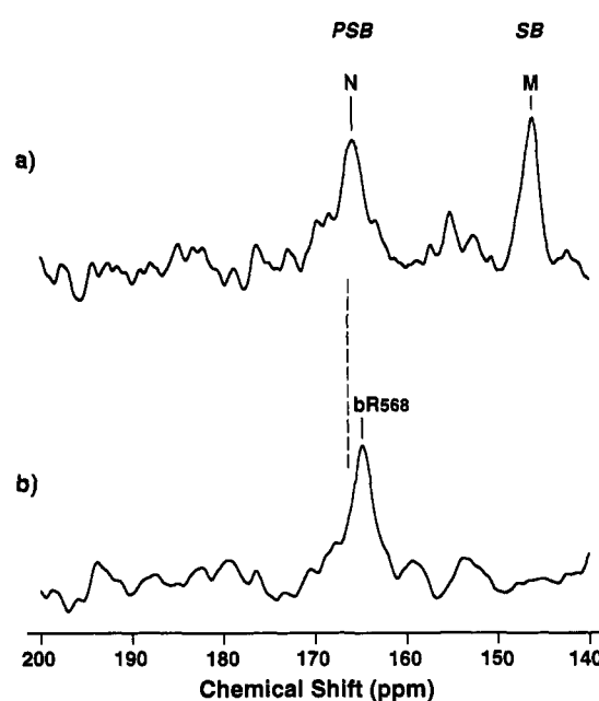
FIGURE 2: 13 C NMR difference spectra of [13- 13 C]retinal bR spinning at 4.5 kHz. (a) The M and N states. (b) The thermal decay product obtained when the sample containing the M and N intermediates is warmed to 0 °C for a couple of minutes and recooled to -50 °C during data acquisition.
